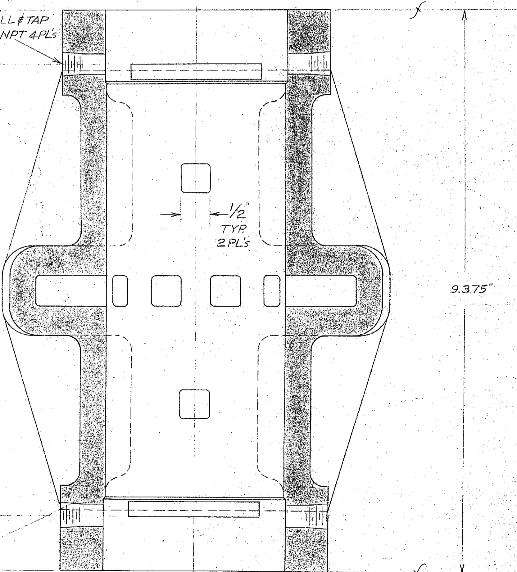
SECTION C-C
